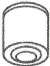
#16 Receiving cup O.D.: 2-1/4" I.O.: 2" Length: 2"
